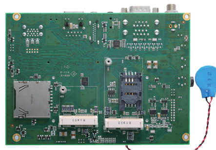
▲ SCM180 Bottom View
