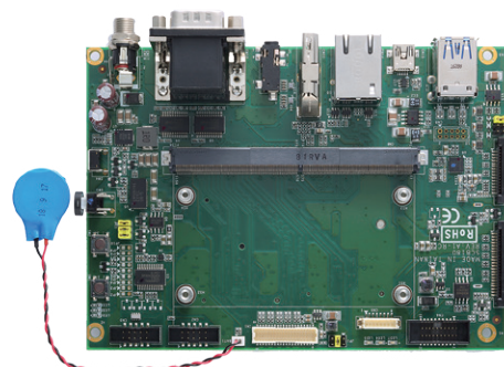
▲ SCM180 Top View
